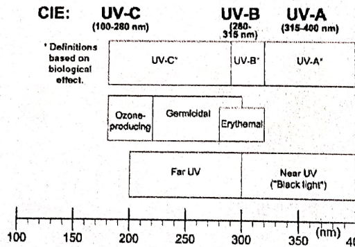
Fig. 1.2 Common ultraviolet band designations.
